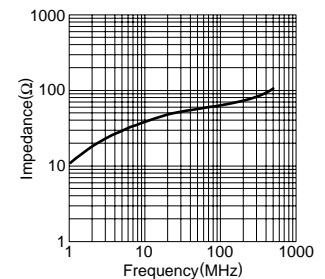
HF70BB6.4X10X3.2
