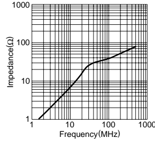
HF40BB5.5X5X2.5
