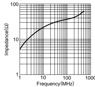
HF70BB6.4X4.5X3.2
