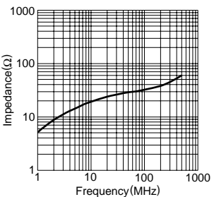
HF70BB6X3.8X3
