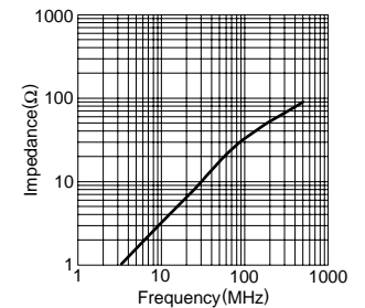
HF30BB3.5X5X1.3
