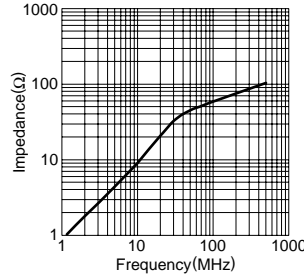
HF40BB5.5X5X2
