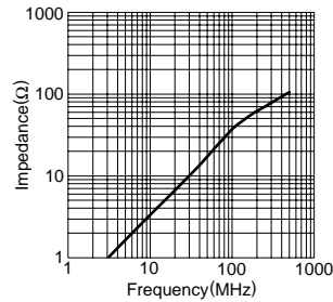
HF30BB3X5X1
