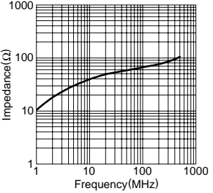
HF70BB9X10X4.5
