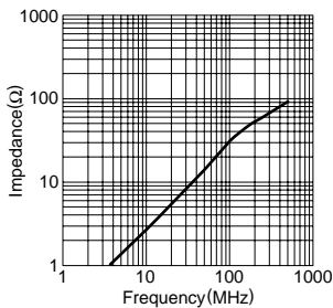
HF30BB5X5X2
