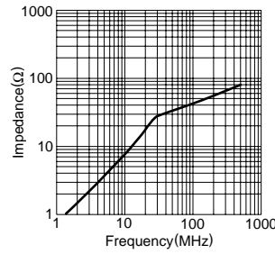
HF40BB5.5X5X2.5
