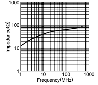
HF70BB4.5X4X2.5
