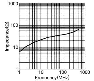
HF70BB5.5X5X2.5
