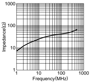
HF70BB5X5X2
