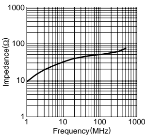
HF70BB4.5X5X1.6
