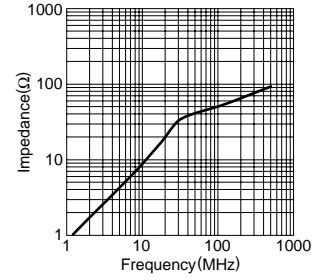
HF40BB6X3.8X3A-G
