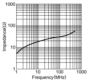
HF70BB6.4X5X3.2
