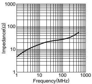
HF70BB3.5X3X1.3
