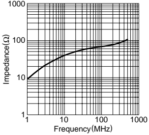
HF70BB9.5X10.4X4.9
