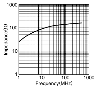
HF70BB4.5X15X1.35
